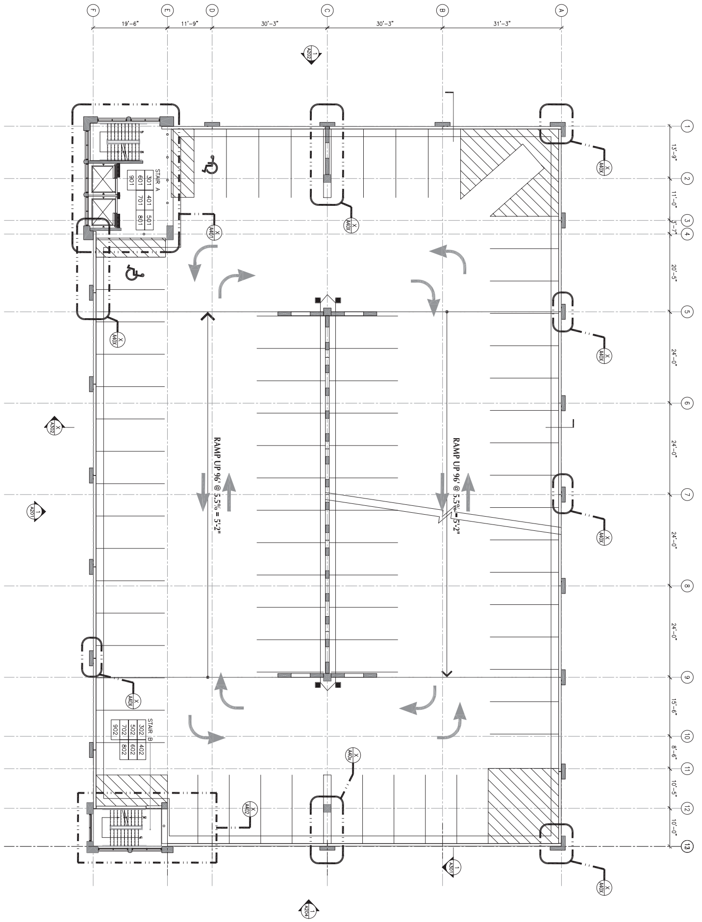
1 TYPICAL FLOOR PLAN - L3-L9 A103 SCALE: 1/8"=1'-0"
