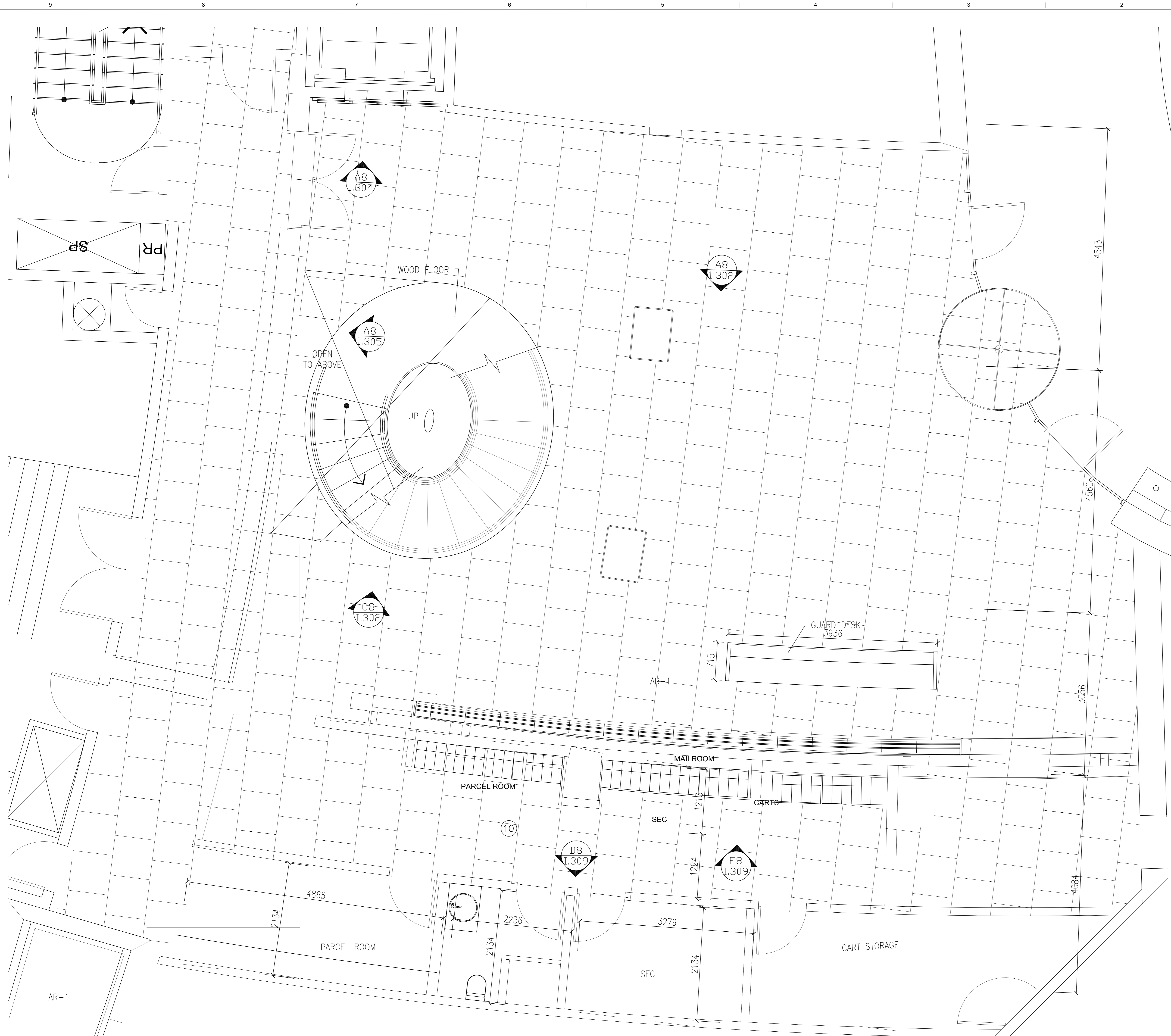
A9 TOWER TWO : LOBBY - CONCOURSE LEVEL Scale: 1/50
