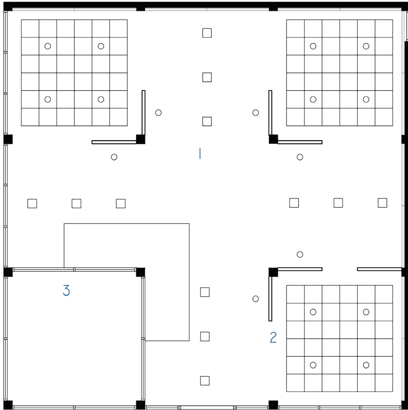
FIRST FLOOR REFLECTED CEILING PLAN
