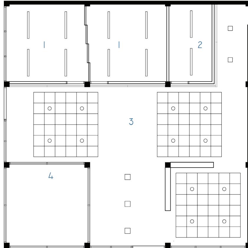
SECOND FLOOR REFLECTED CEILING PLAN
