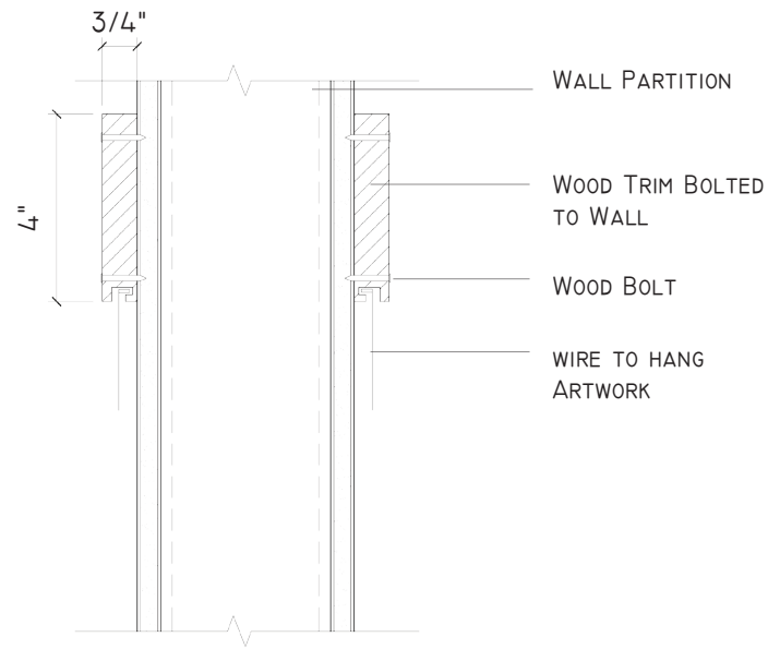
GALLERY WALL PARTITION DETAIL
