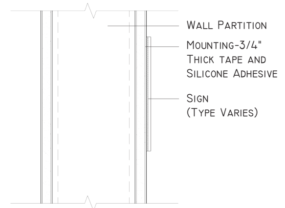
SIGNAGE DETAIL
