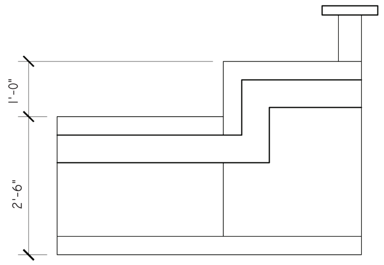
RECEPTION DESK SIDE ELEVATION
