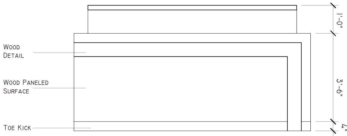
RECEPTION DESK FRONT ELEVATION
