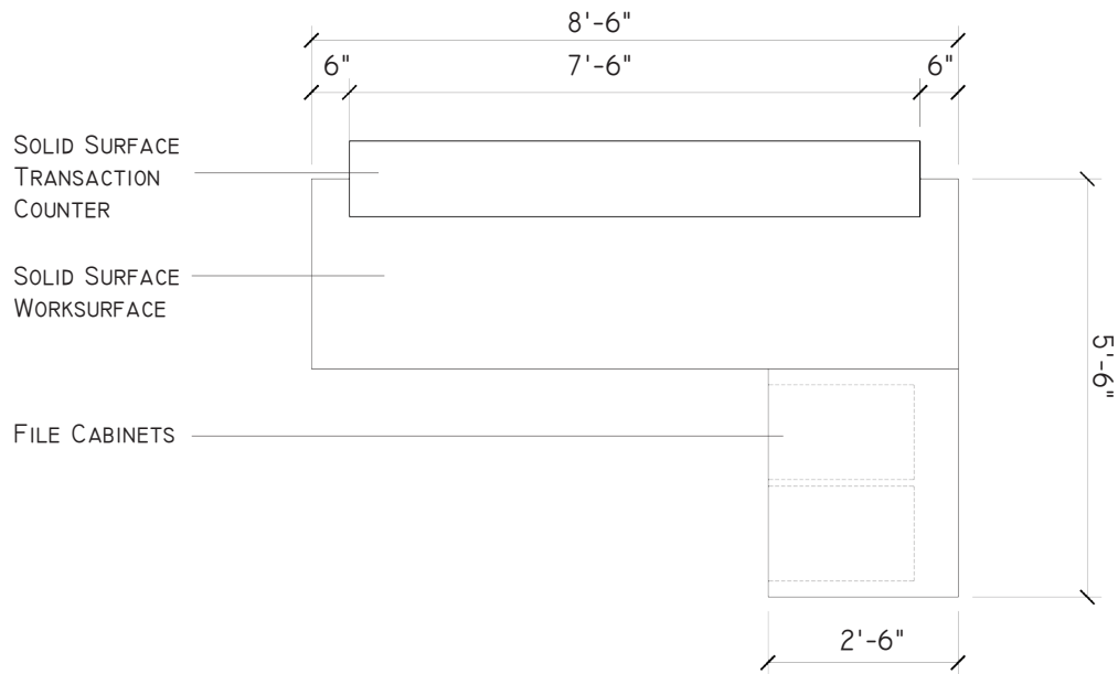
RECEPTION DESK PLAN
