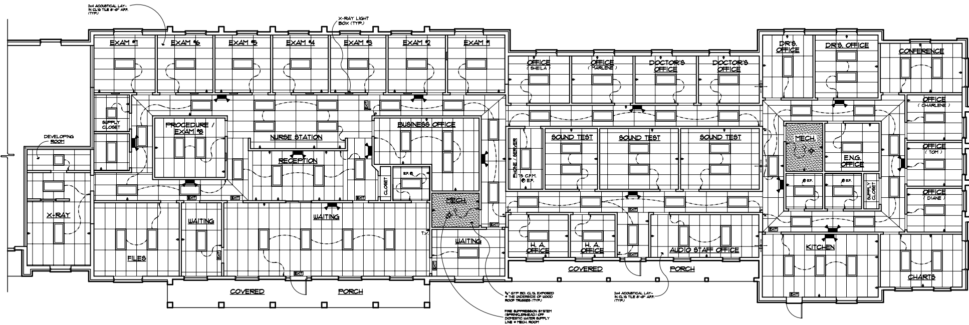
REFLECTED CEILING / ELECTRICAL PLAN SCALE: 3/16" = 1'-0"
