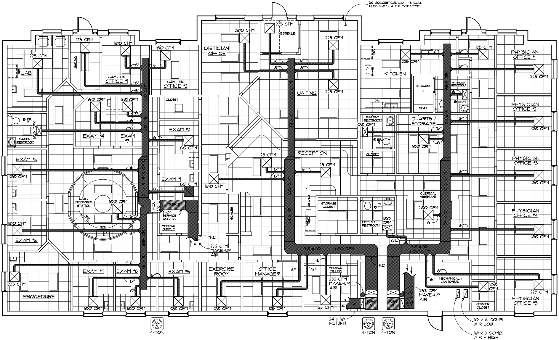
MECHANICAL / H.V.A.C. PLAN SCALE: 3/16" = 1'-0"
