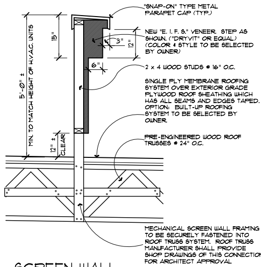
A802 A5 SCREEN WALL CONNECTION DETAIL SCALE: 3/4" = 1'-0"
