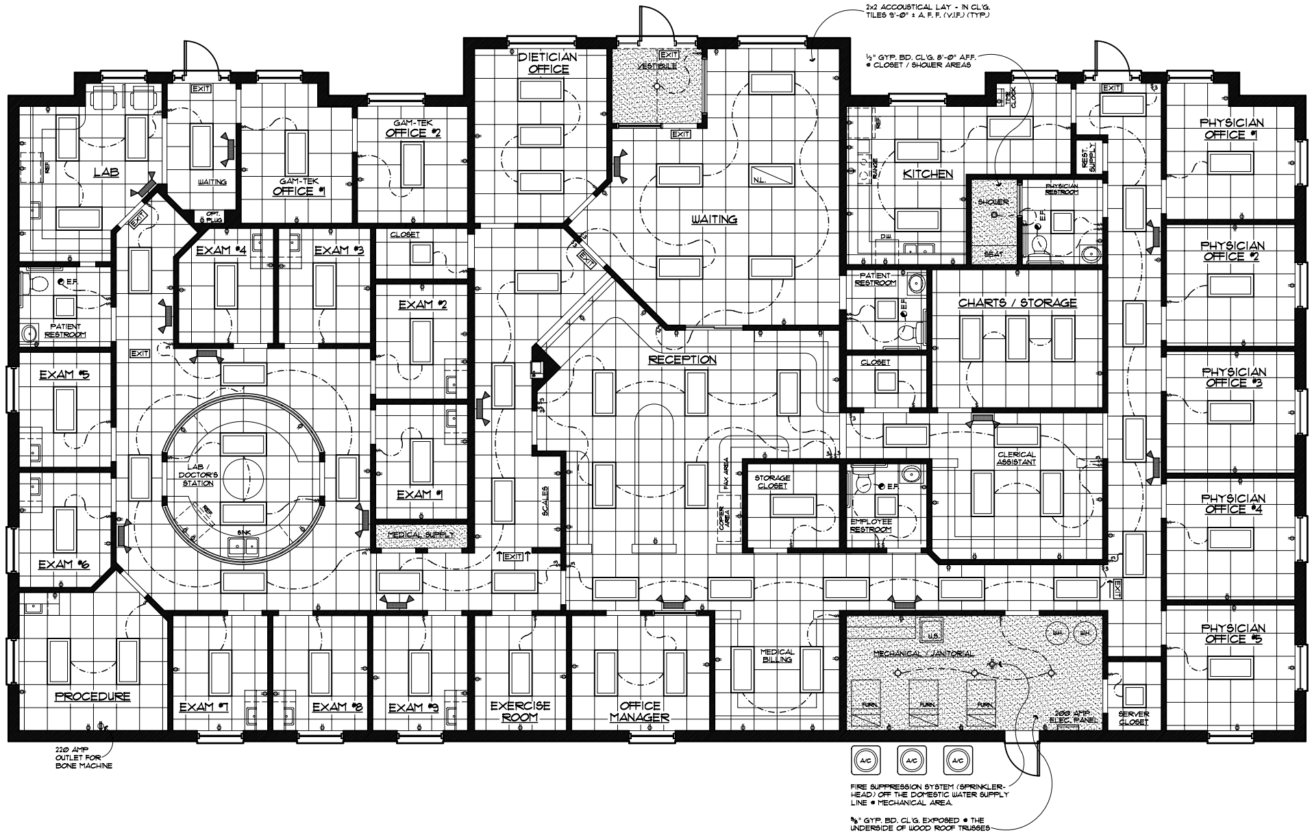
ELECTRICAL / REFLECTED CEILING PLAN SCALE : 3/16" = 1'-0"
