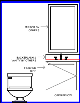
POWDER BATH ELEVATION
