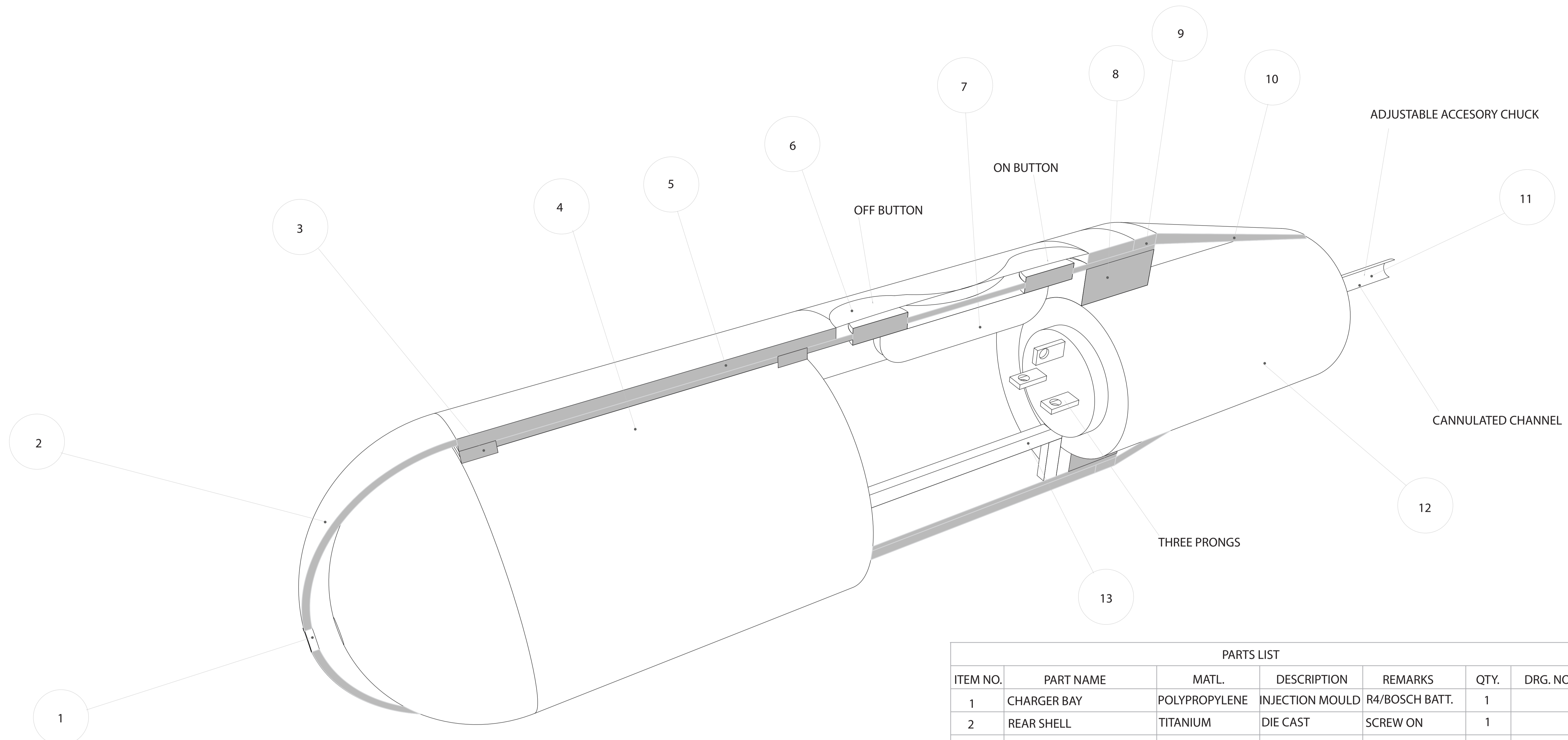
ISOMETRIC CROSS-SECTION OF NEUTRO+ ALL CROSS-SECTIONS ARE SHADED OMITTED CROSS-SECTIONS FOR PART 4,12 AS THEY ARE STANDARD PARTS
