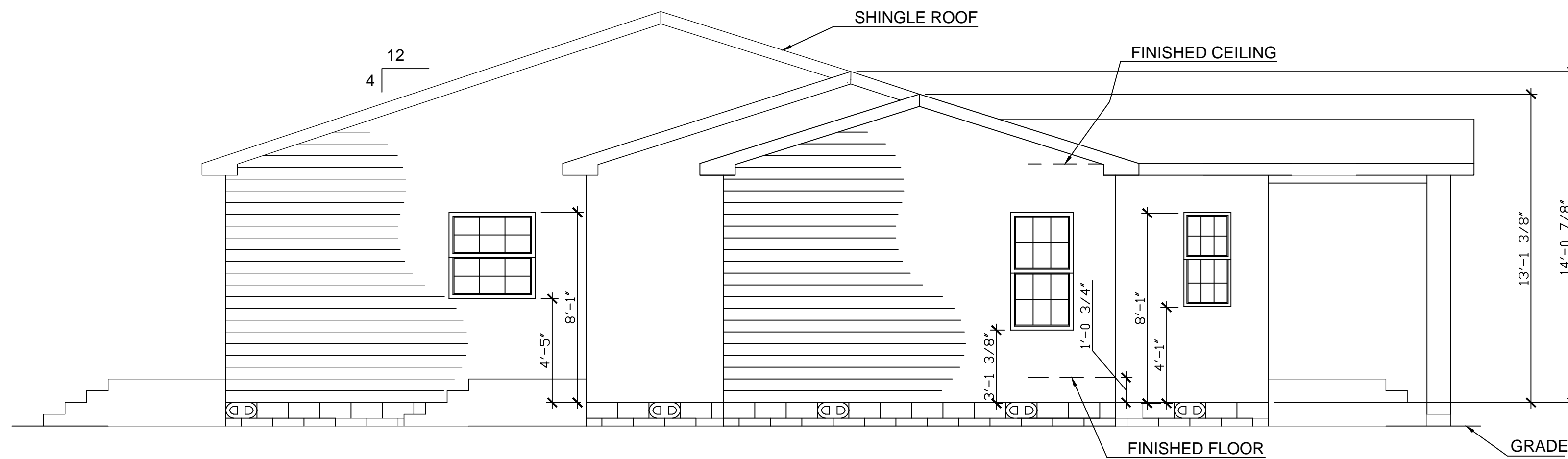
ELEVATION PLAN SCALE: 1/4" = 1'-0"
