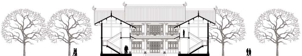
B - B Section Plan
