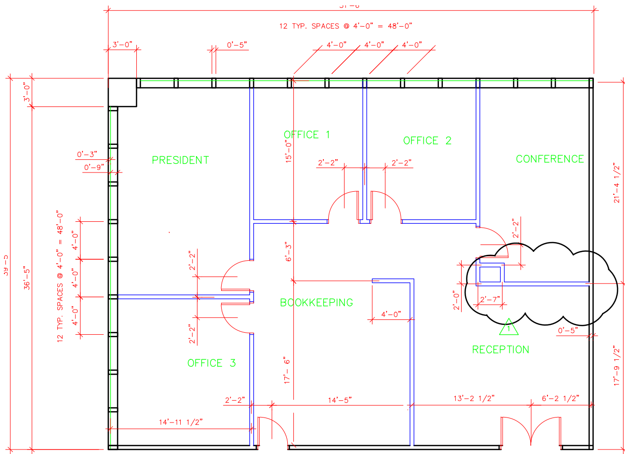
TENANT SPACE FLOOR PLAN SCALE: 1/8" = 1'-0"
