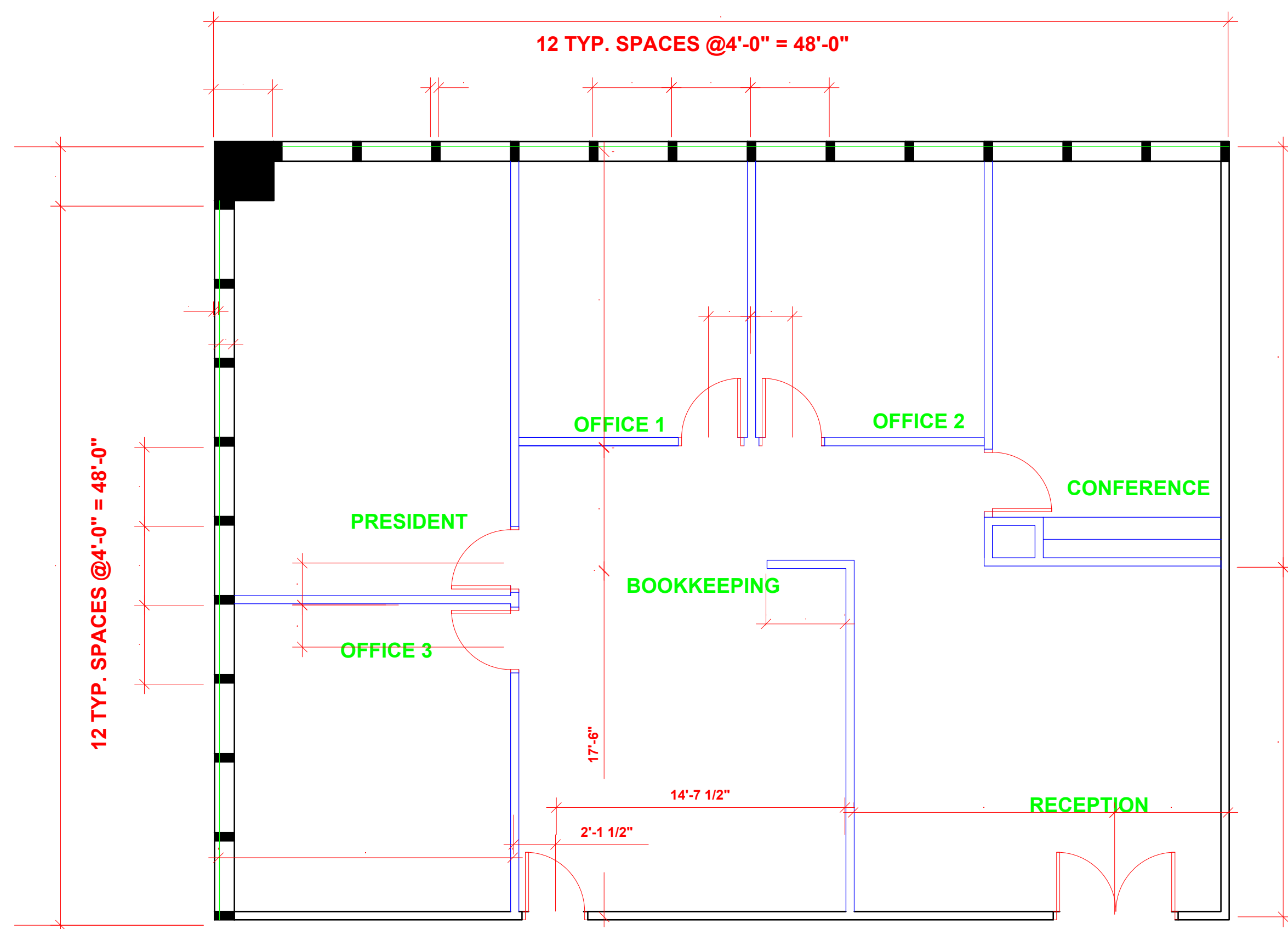
FLOOR PLAN
