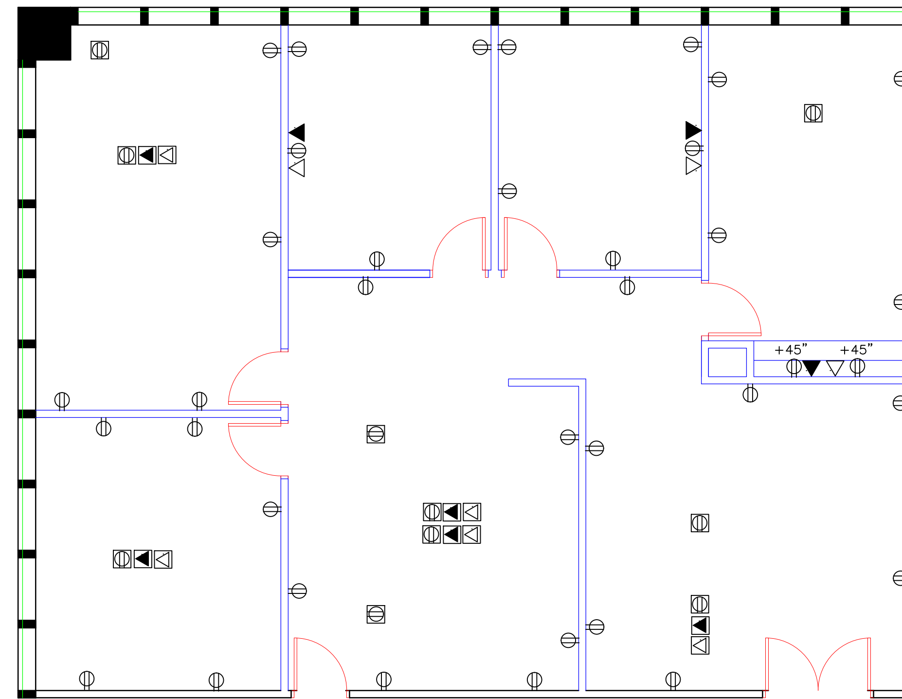
VOICE/DATA/POWER PLAN
