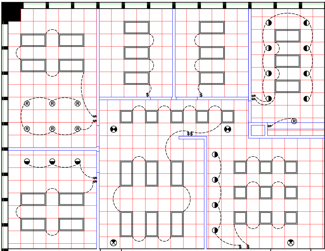
REFLECTED CEILING PLAN SCALE: 1/8" = 1'-0"
