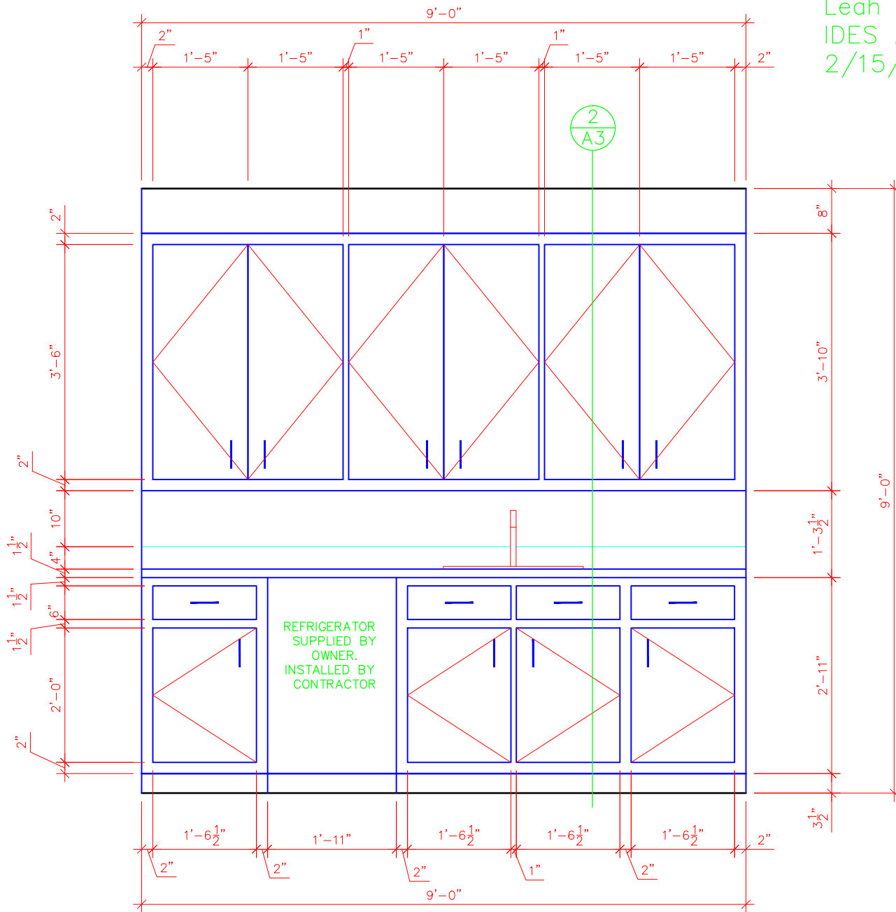
1 CONFERENCE ROOM CABINET ELEVATION SCALE: 1/2"=1'-0"
