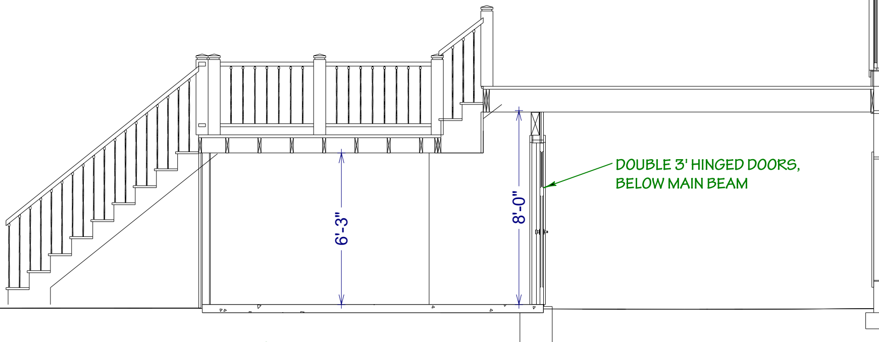
Section View of Optional Storage Closet @ 1/4" = 1' - 0"
