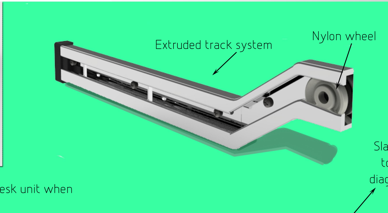
Transparent outer unit used for illustration purposes
