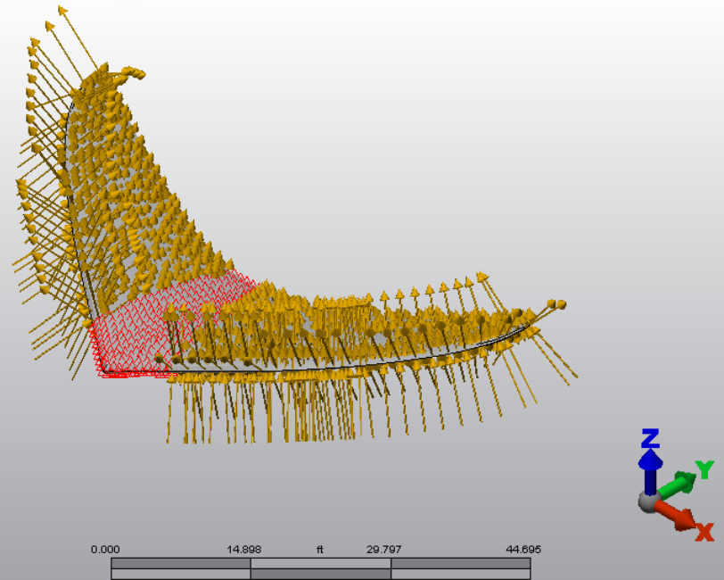
Applied Load with Constrained Center
