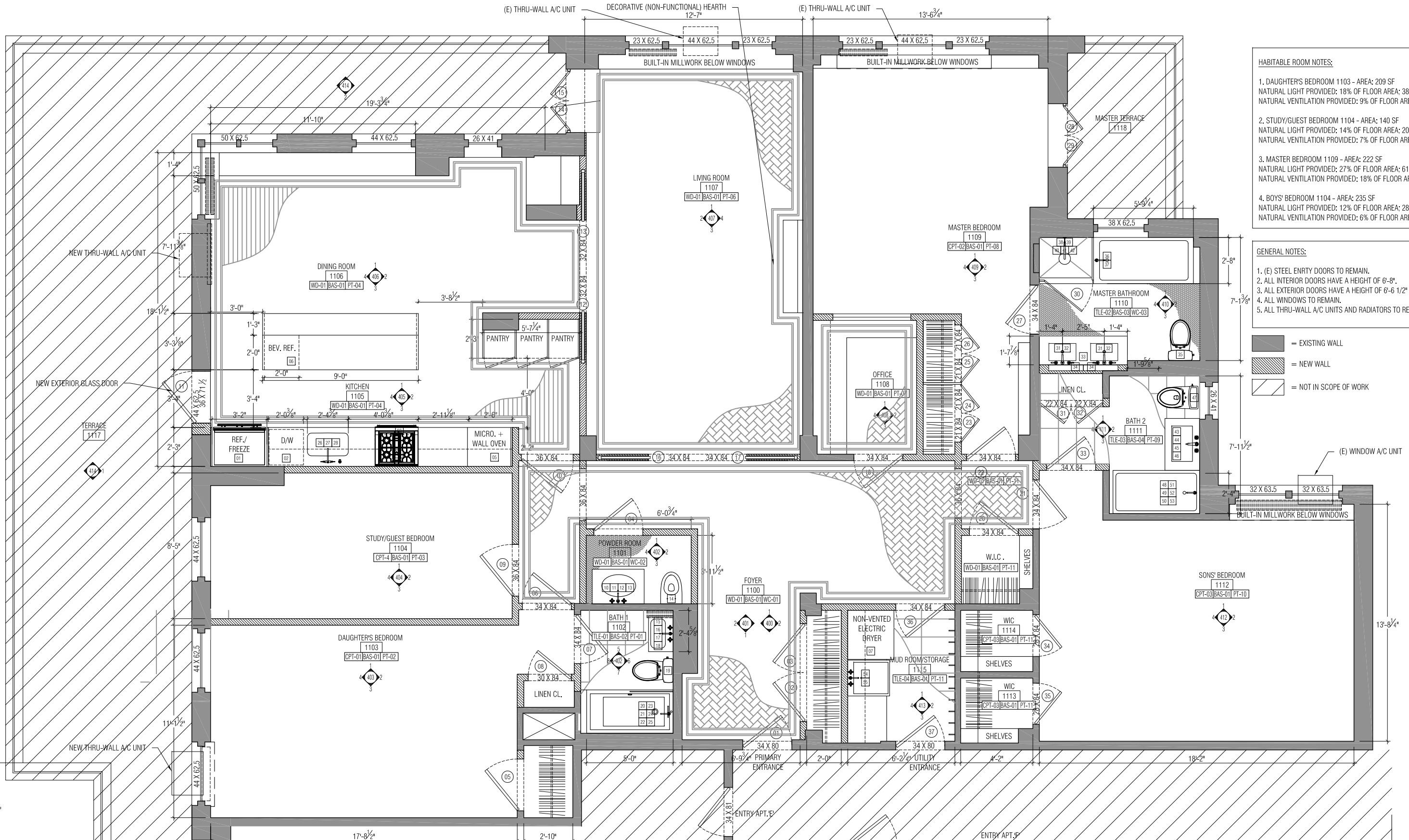
1 APT. 11CD - CONSTRUCTION PLAN SCALE: 3/16" = 1'-0"
