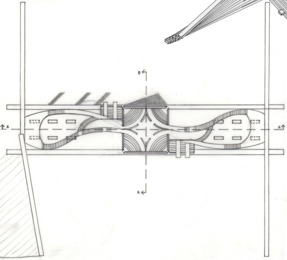
Floor Plan
