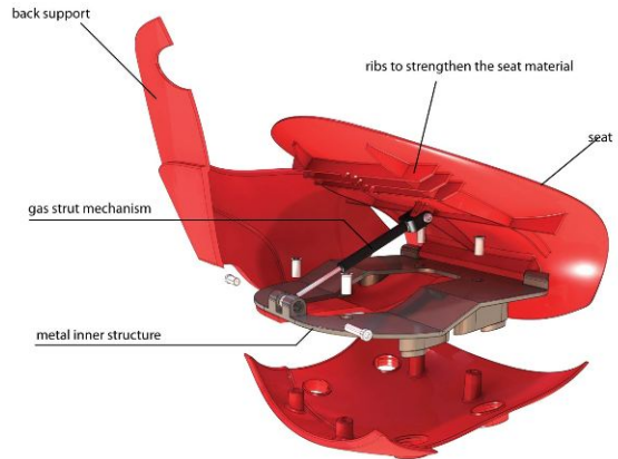
Solidworks rendering showing section details
