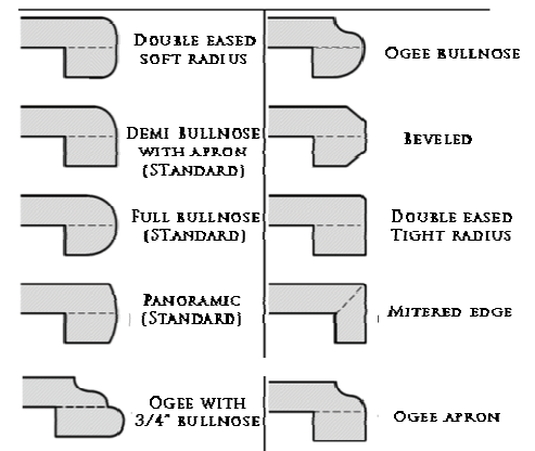
SAMPLES OF POSSIBLE EDGE DETAILS
