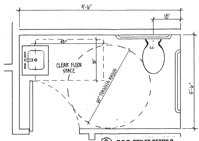
(C) A.D.A. TOILET DETAILS
