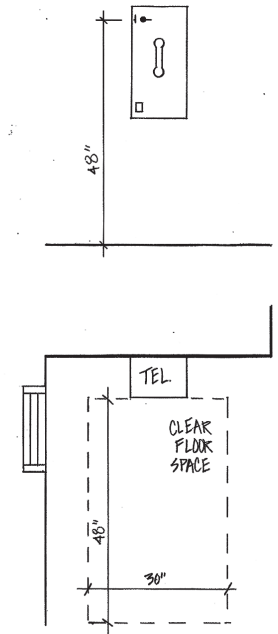
(B) A.D.A. PHONE DETAILS
