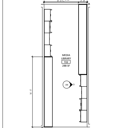
2 MEDIA LIBRARY A2 1/4" = 1'-0"
