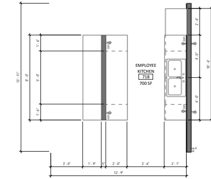
1 EMPLOYEE KITCHEN A2 3/8" = 1'-0"
