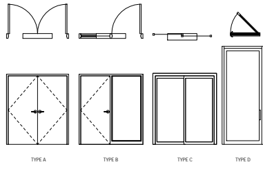
DOOR TYPES 1/4" = 1'-0"
