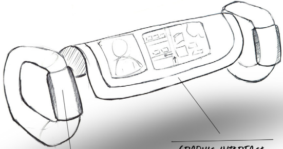
GRAPHIC INTERFACE
