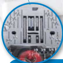
Superior Feed System contacts the fabric at 7 specific points
