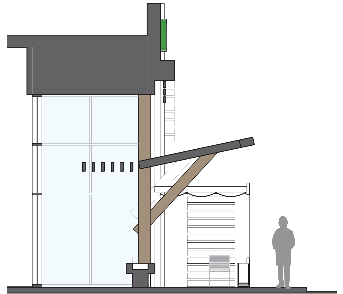
SEATING AREA SECTION
