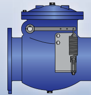
Lever & Spring
