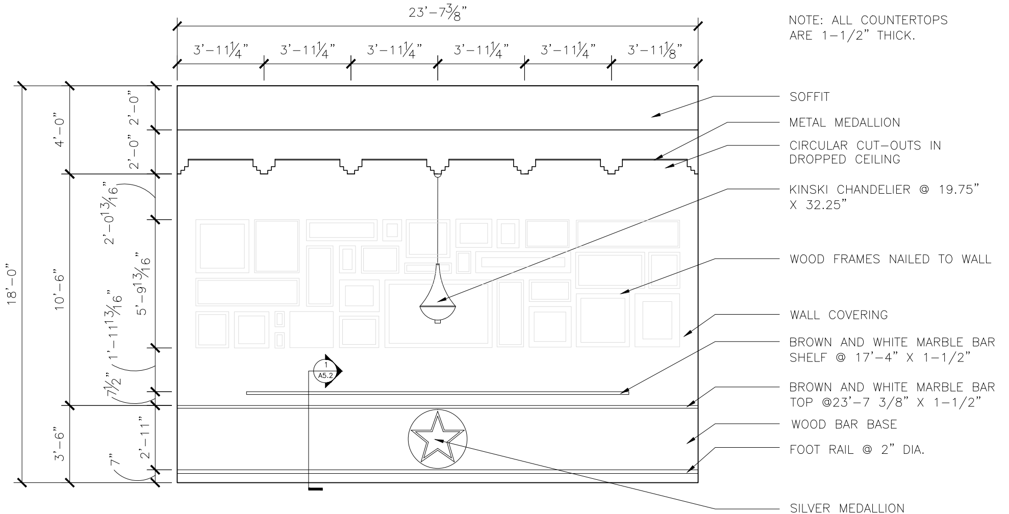
1 RESTAURANT BAR ELEVATION SCALE: 1/2"=1'-0"
