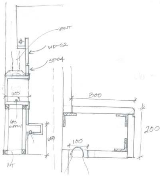
SECTION AT FIREPLACE
