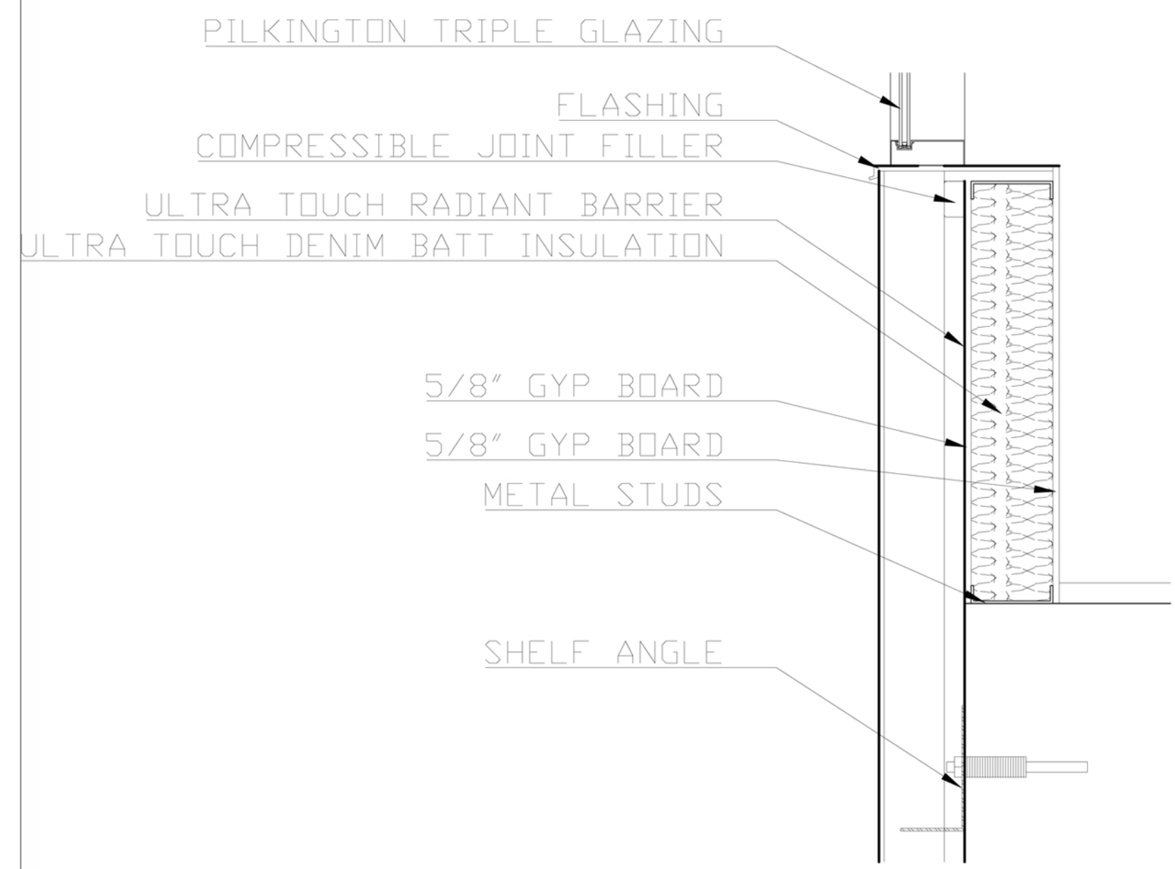
Detail Two Scale: 1" = 1' - 0"
