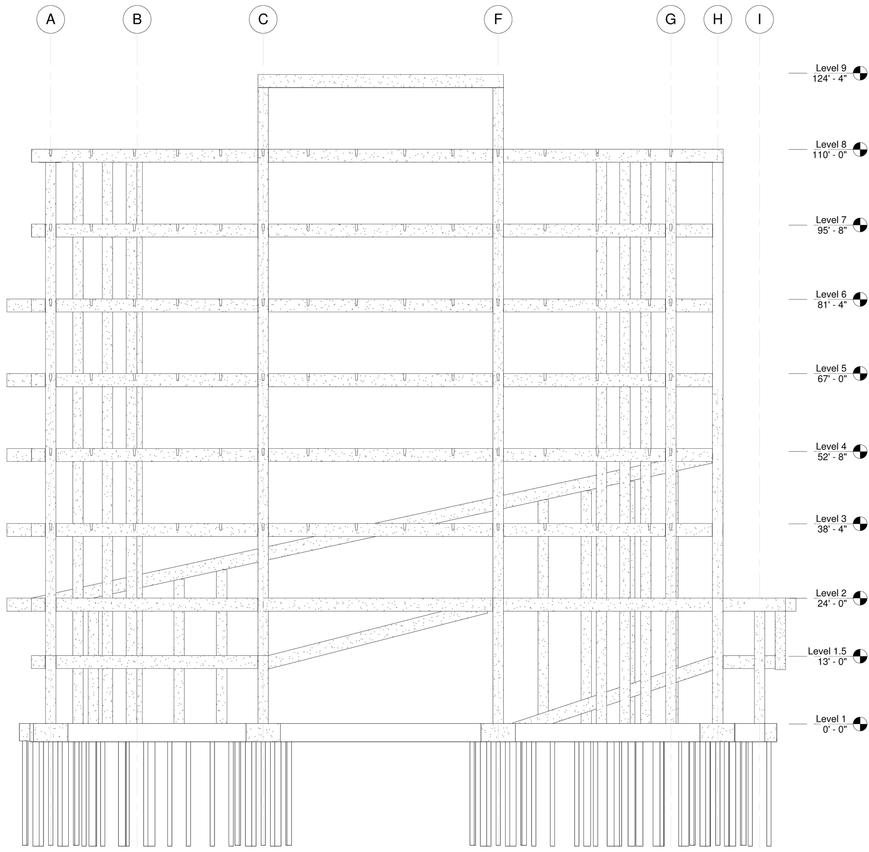
Scale: 3/32"=1' South Structural Elevation
