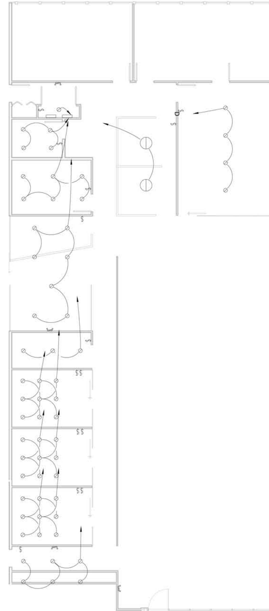
277V Lighting Plan [Panel B]
