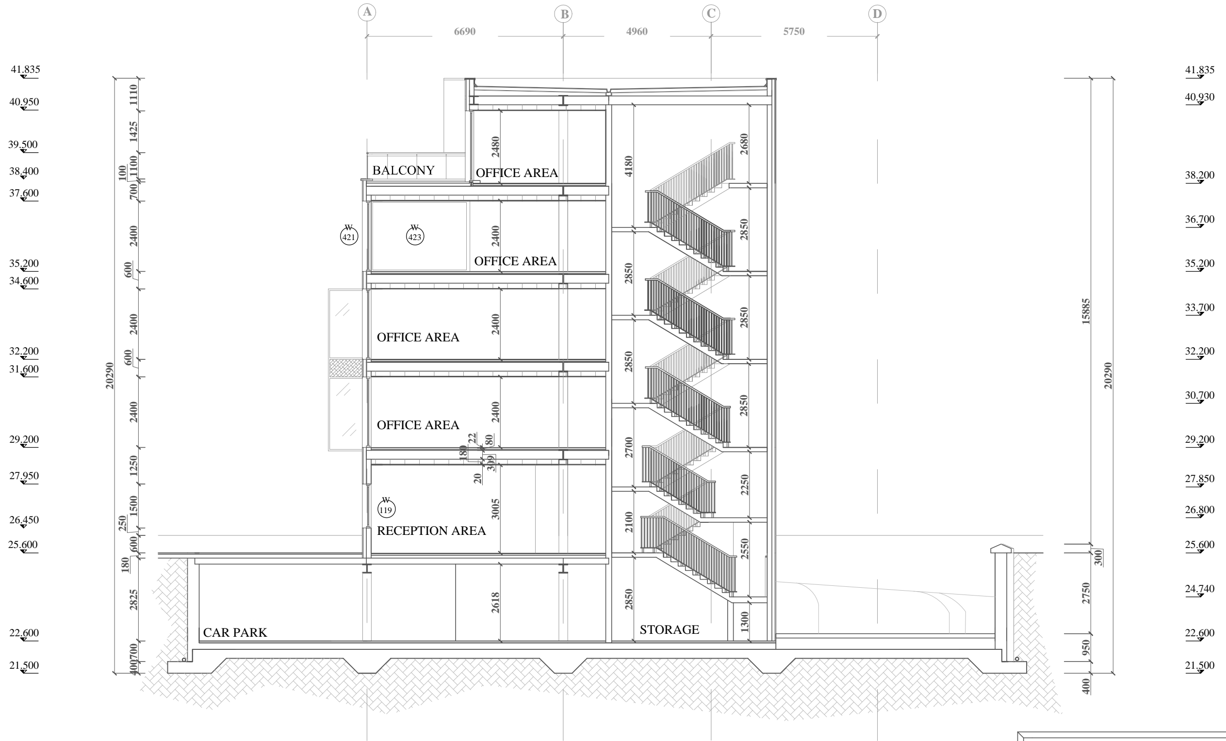
5 SECTION B-B SCALE 1:125
