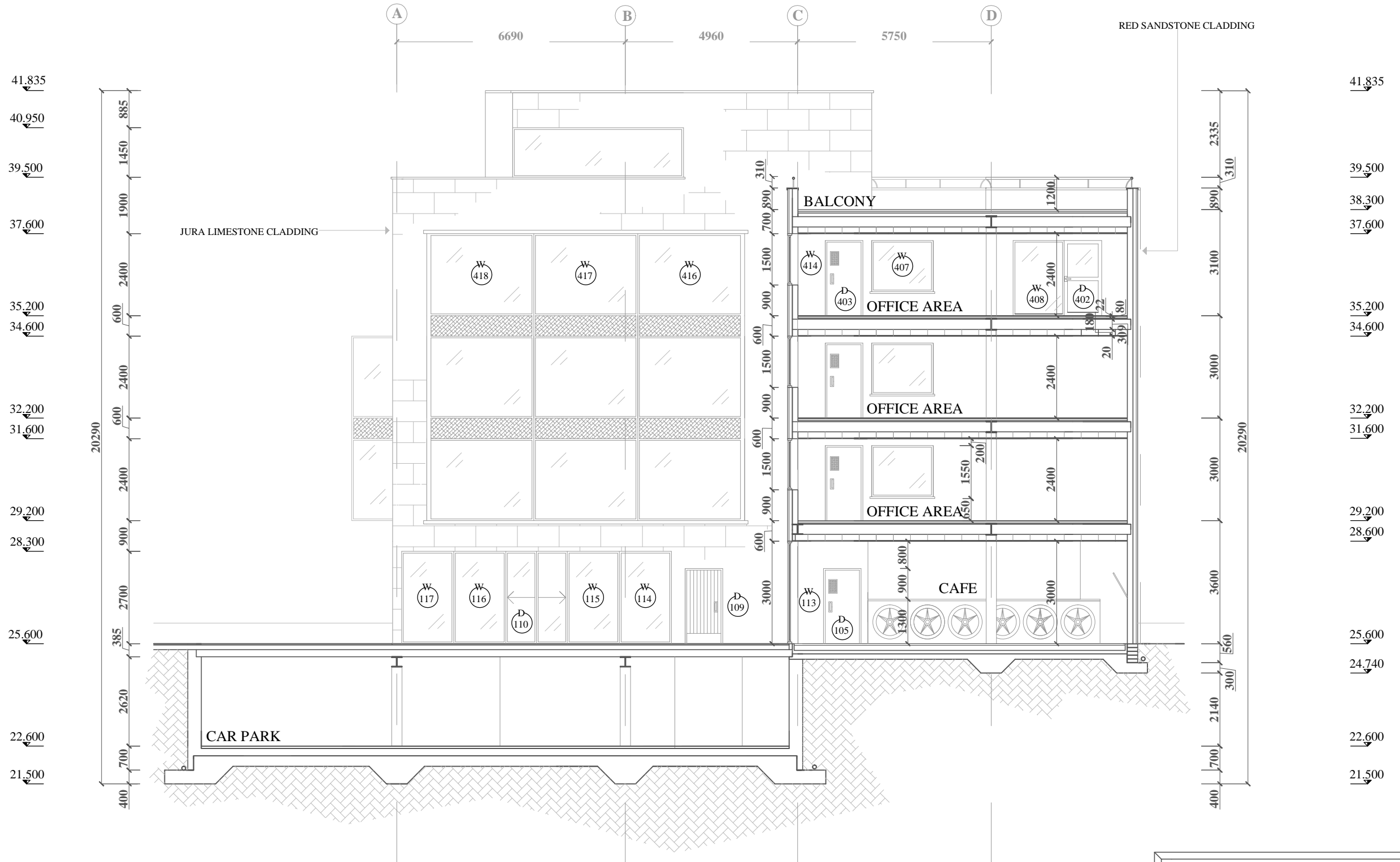
4 SECTION A-A SCALE 1:125
