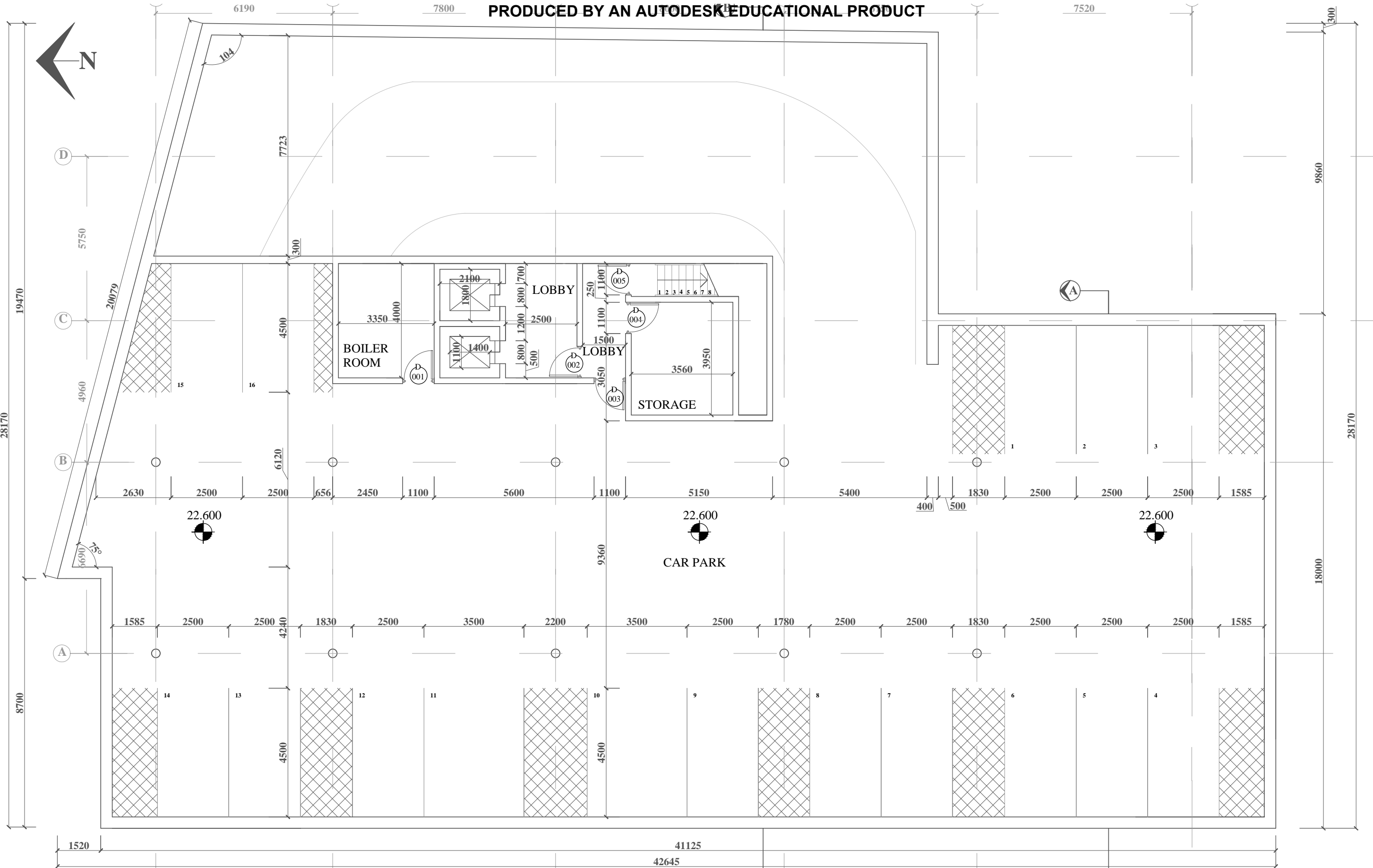
1 BASEMENT FLOOR PLAN SCALE 1:125
