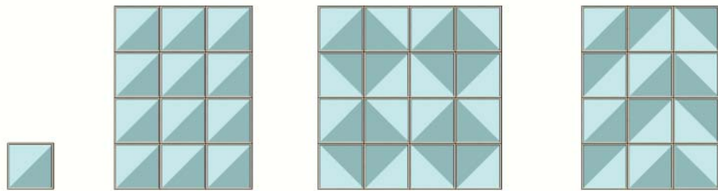
SINGLE BOX CONFIGURATIONS
