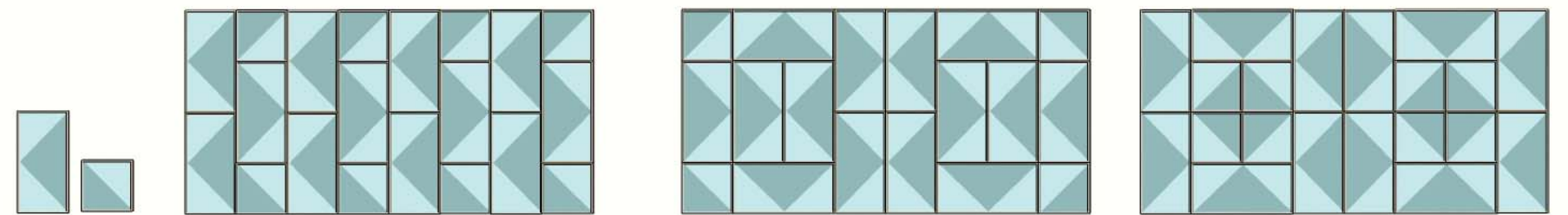
DOUBLE BOX CONFIGURATIONS
