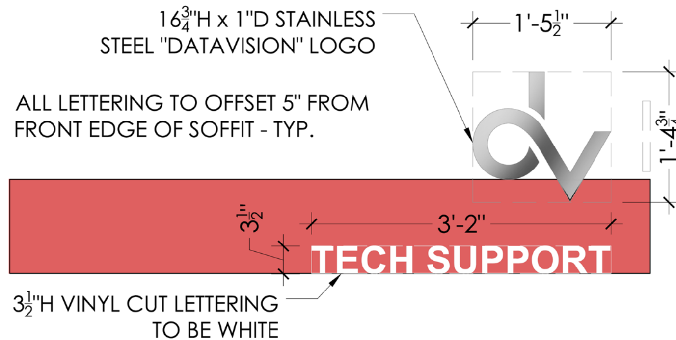
B1 - PARTIAL NORTH ELEVATION_POS SOFFIT_SIGNAGE
