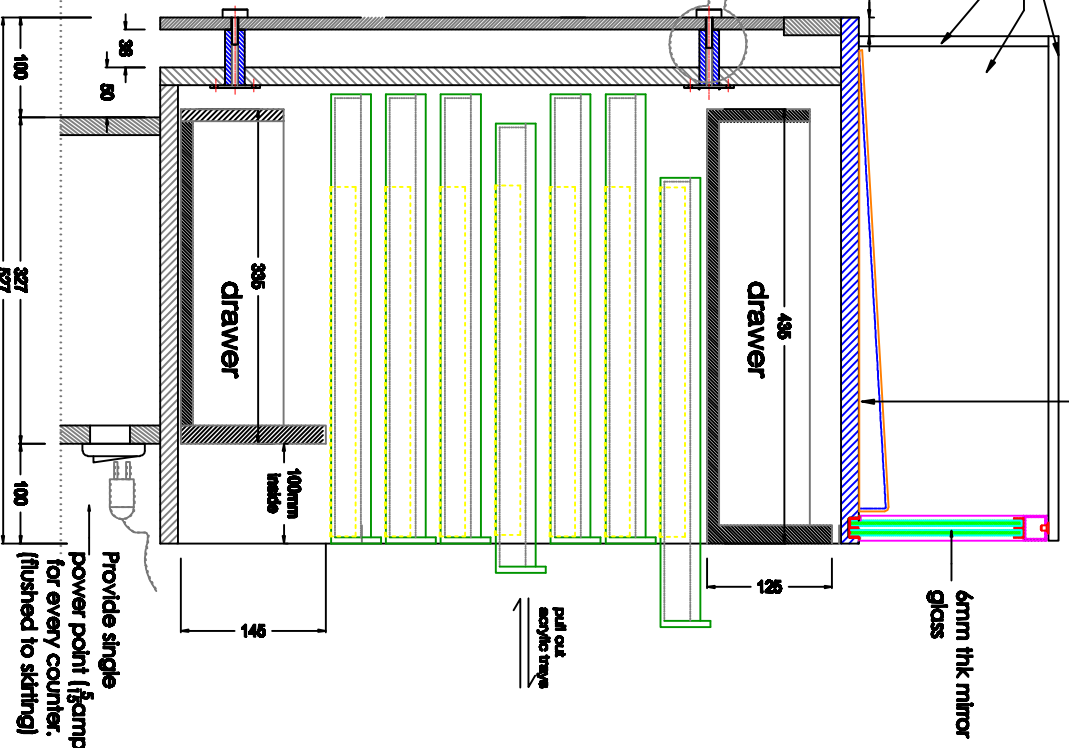
Section - XX' (SCALED UP FOR CLARITY)
