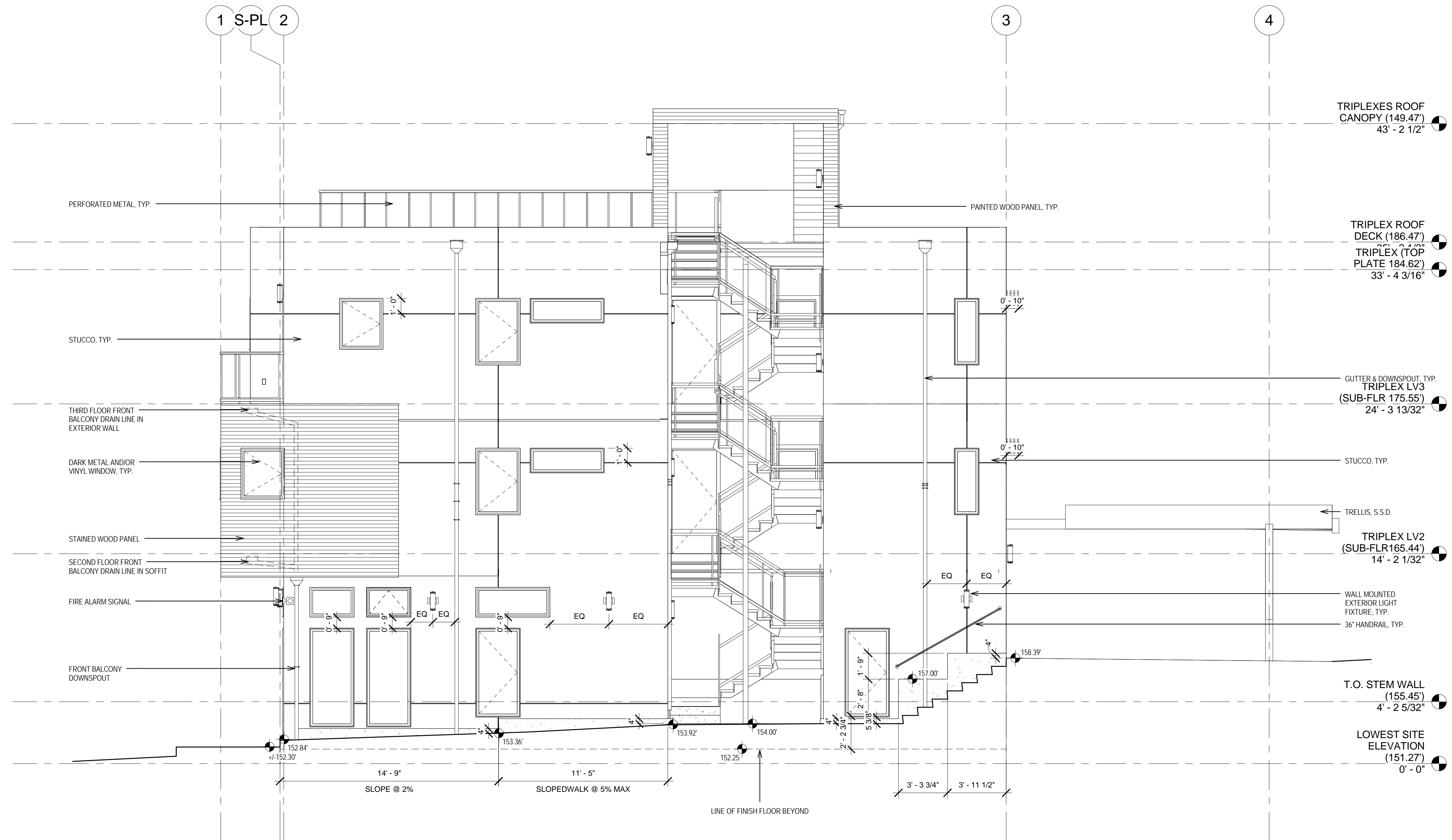
1 LOT 3 - EAST ELEVATION SCALE: 1/4" = 1'-0"
