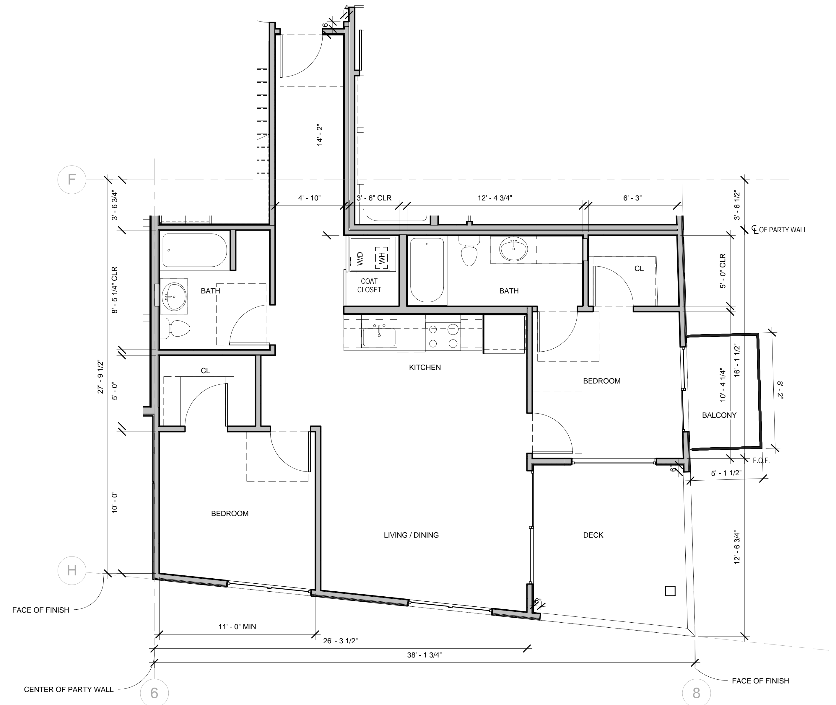
2 UNIT 9 - RESIDENTIAL 2 BR. SCALE: 1/4" = 1'-0"
