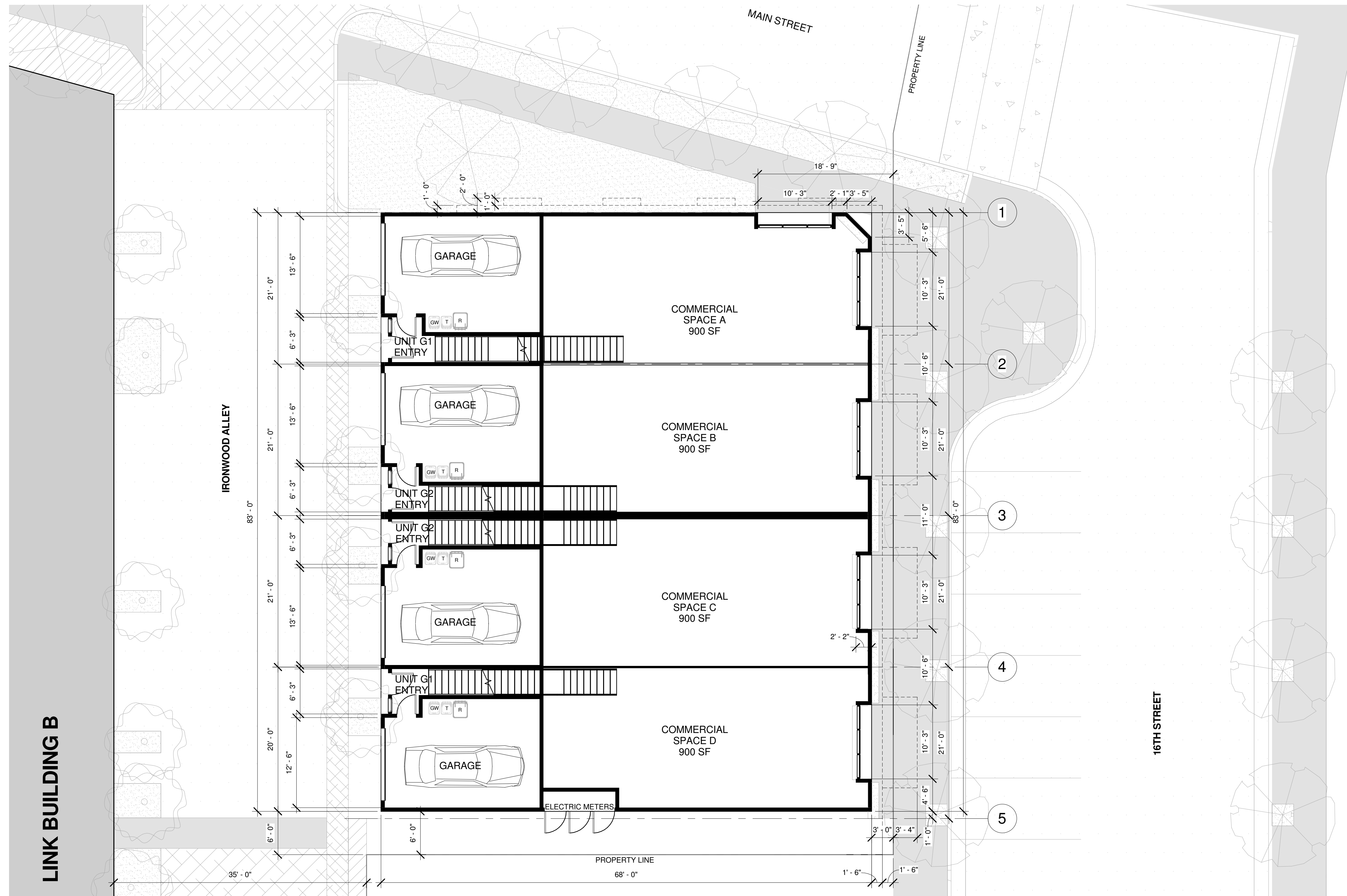
1 GROUND FLOOR AND SITE PLAN SCALE: 1/8" = 1'-0"
