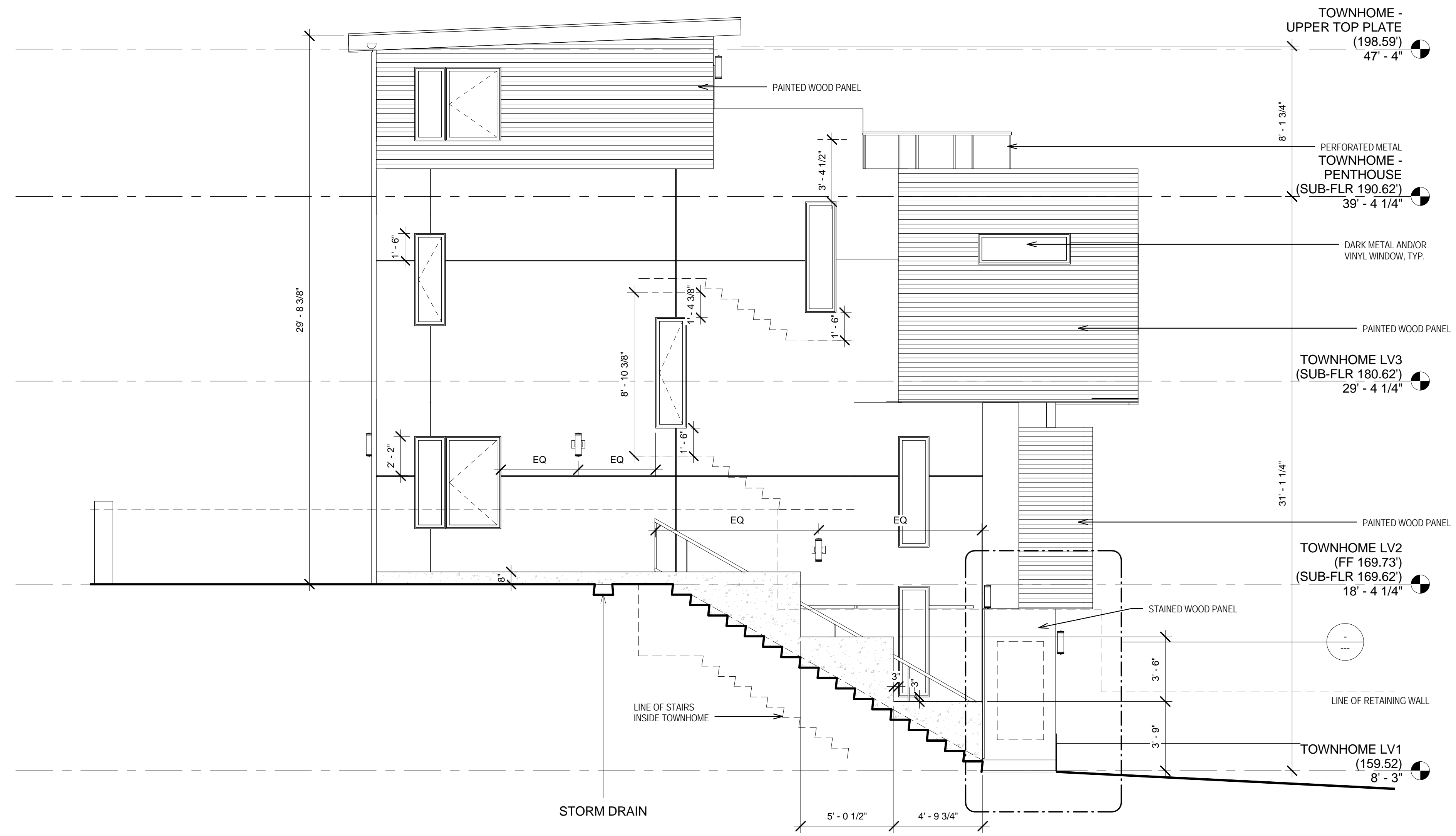
1 TOWNHOME WEST ELEVATION SCALE: 1/4" = 1'-0"
