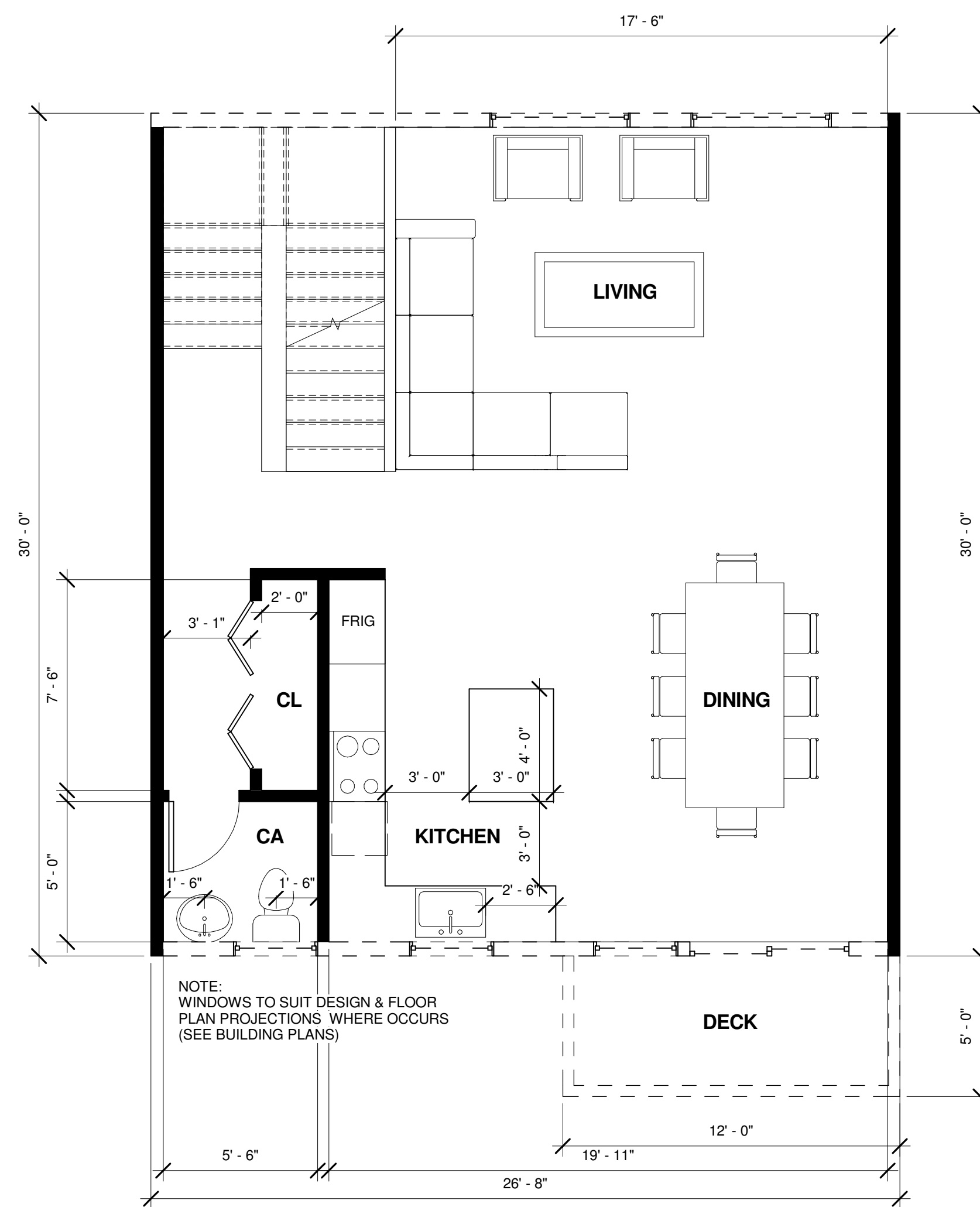
2 UNIT C1 LEVEL 2 SCALE: 1/4" = 1'-0"
