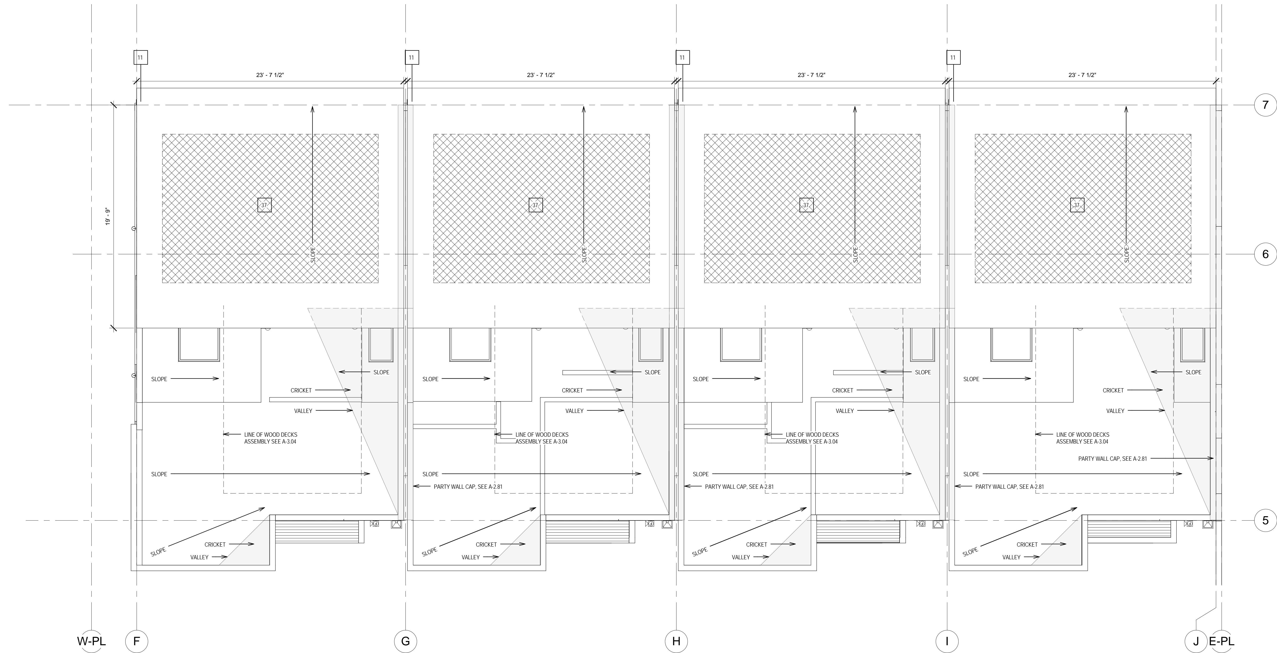
1 TOWNHOME - ROOF PLAN 1/4" = 1'-0"
