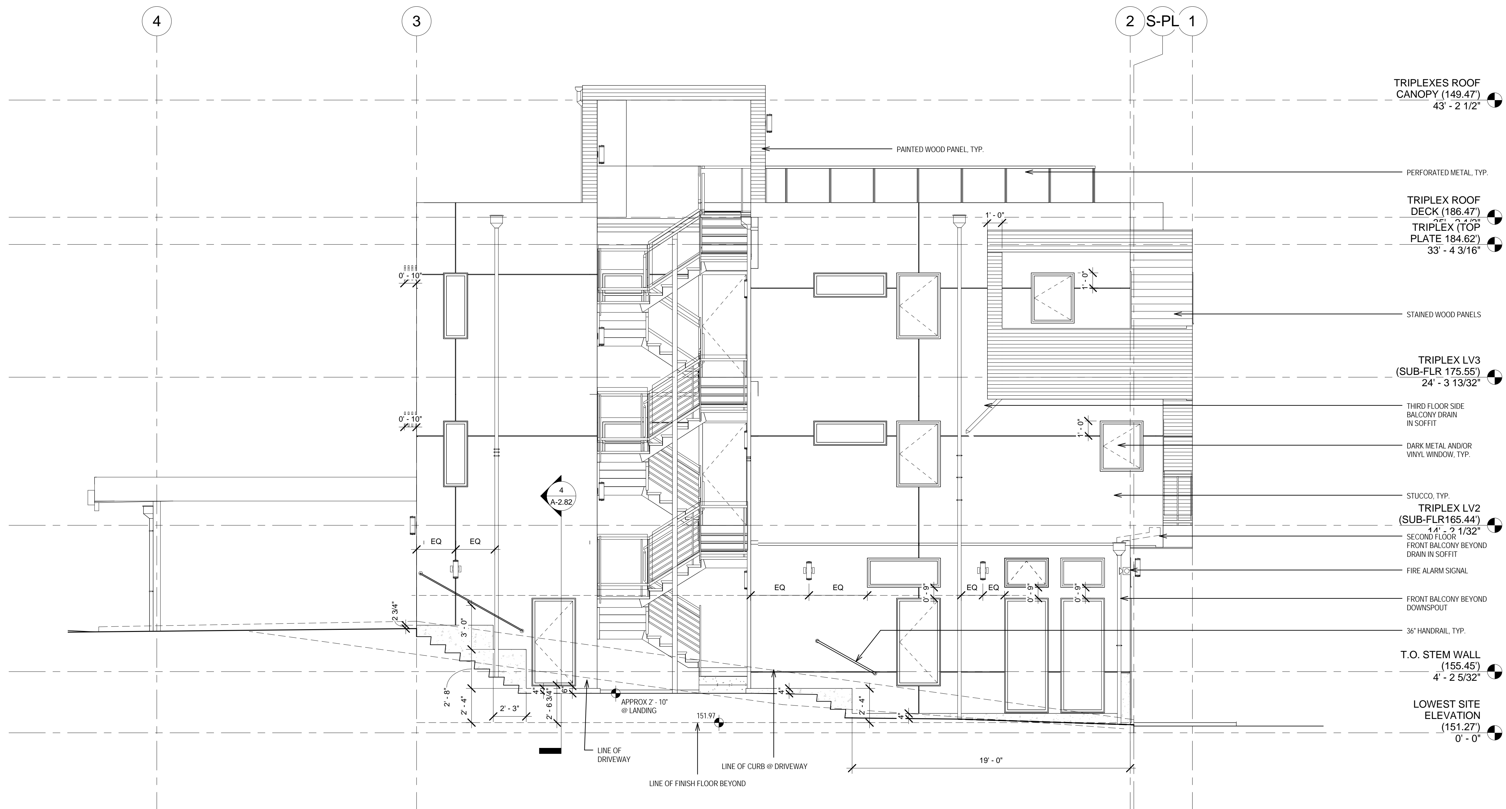
1 LOT 2 - EAST ELEVATION SCALE: 1/4" = 1'-0"
