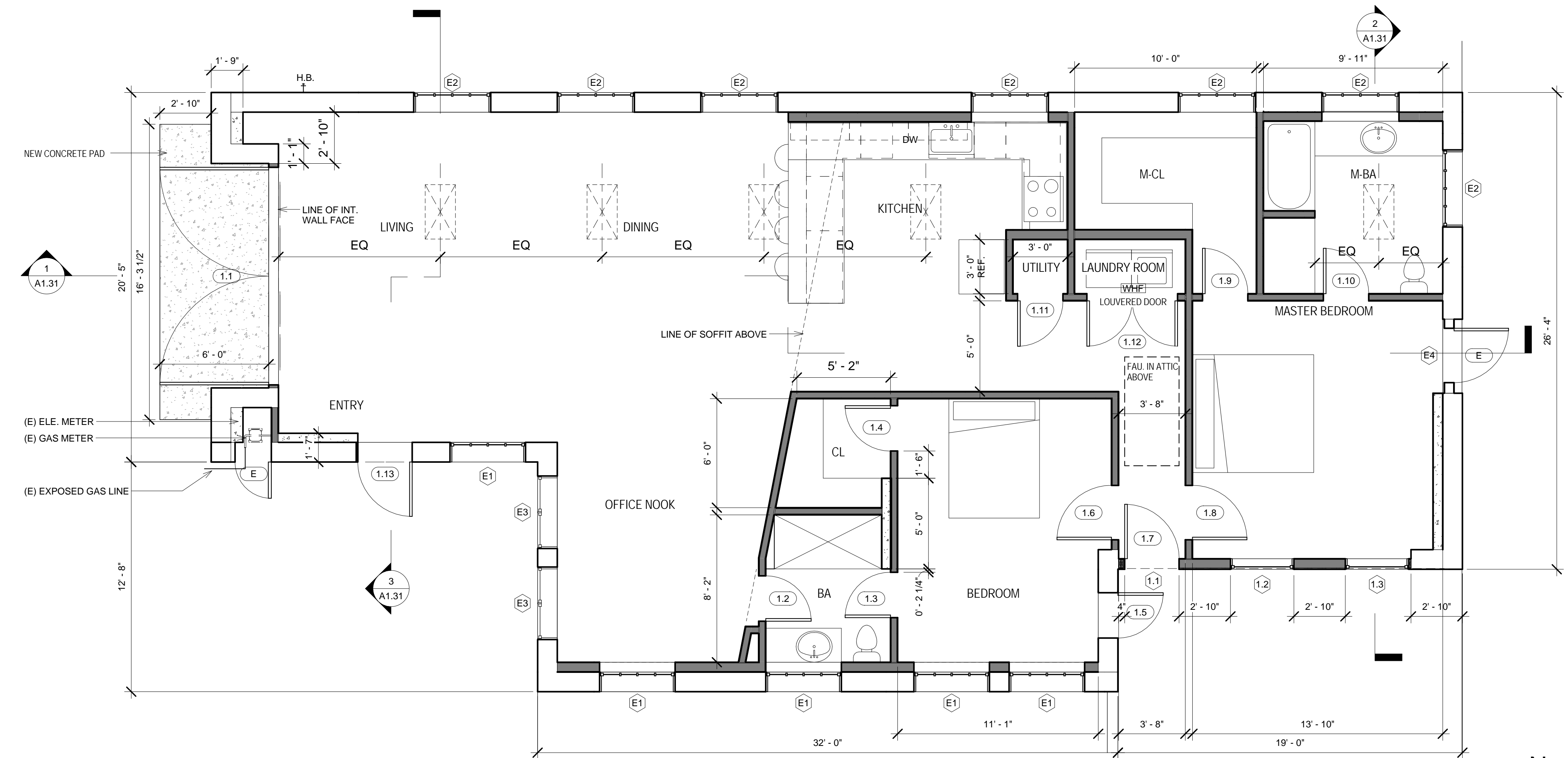
1 LEVEL 1 - PROPOSED FIREHOUSE SCALE: 1/4" = 1'-0"
