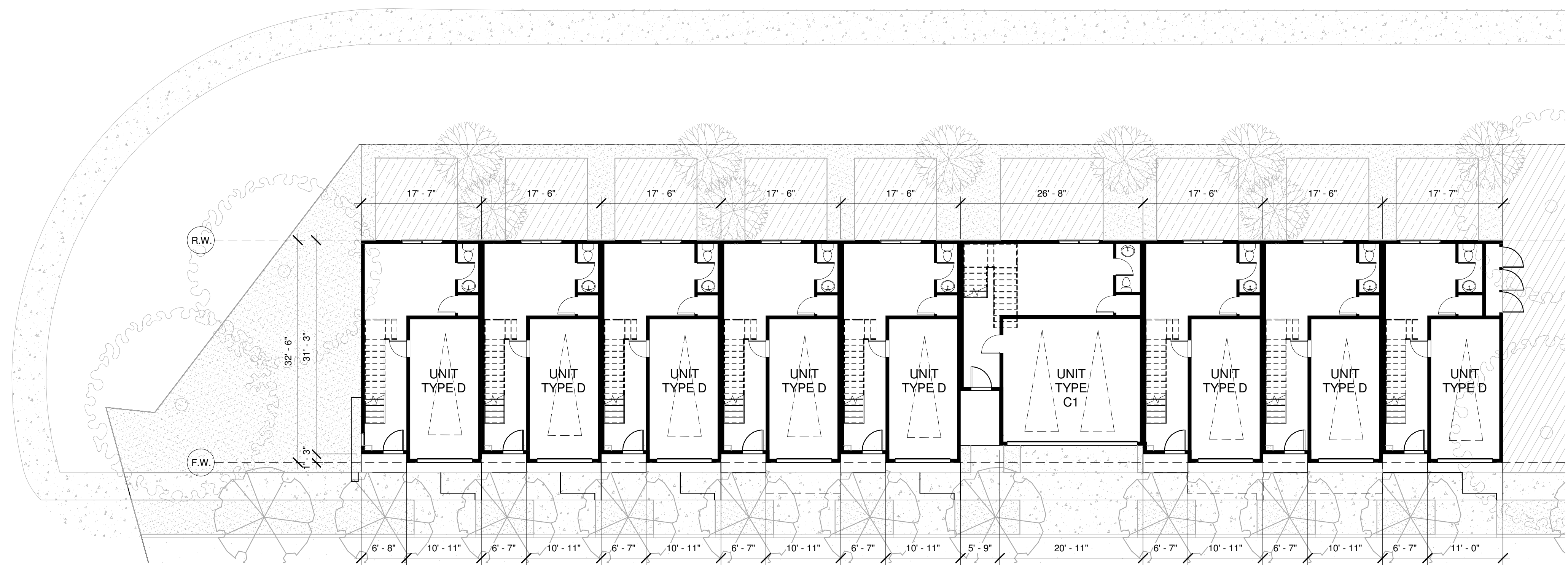
1 MOVE (A) - GROUND FLOOR SCALE: 3/32" = 1'-0"
