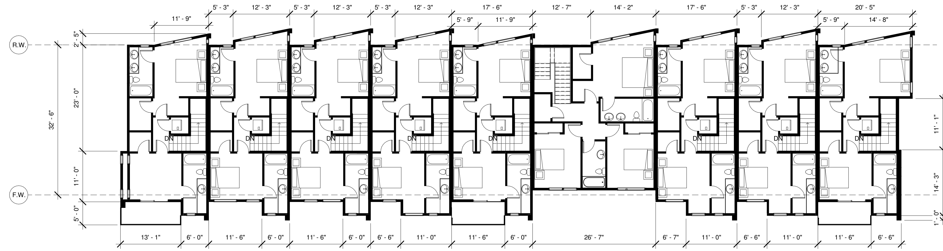
3 MOVE (A) - 3RD FLOOR SCALE: 3/32" = 1'-0"
